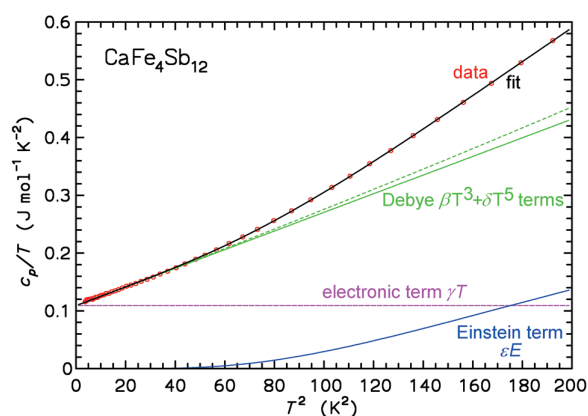
Figure 4: Specific heat capacity of \text{CaFe}_4\text{Sb}_{12} below 14.1 K. The lines give the contributions of the individual terms of the fit to the model (see text).
