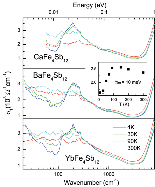
Fig. 9: Spectra of the optical conductivity \sigma_1(\omega, T) at selected temperatures below and above T \approx 90 K, where a pseudogap forms below \approx 17 meV. For \text{BaFe}_4\text{Sb}_{12} the inset shows \sigma_1(\omega, T) at \hbar\omega = 10 meV, demonstrating the evolution of the pseudogap.
