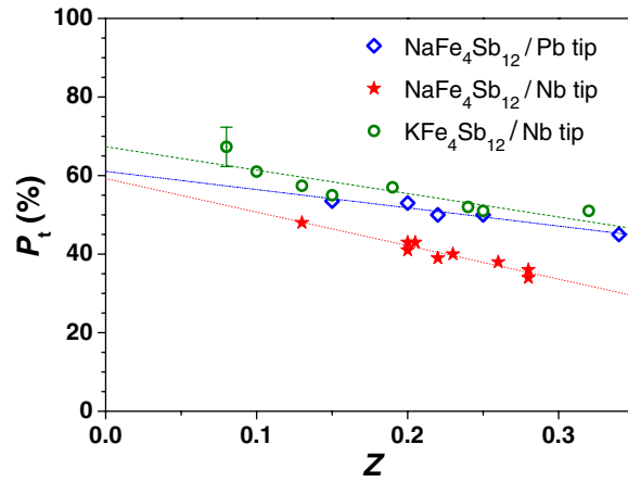
Fig. 12: Transport spin polarization P_t in dependence on the Z -value for the different sample/tip combinations measured. The extrapolation to zero Z yields the intrinsic spin polarization of the two skutterudites. The indicated error bar is representative for all measurements.
