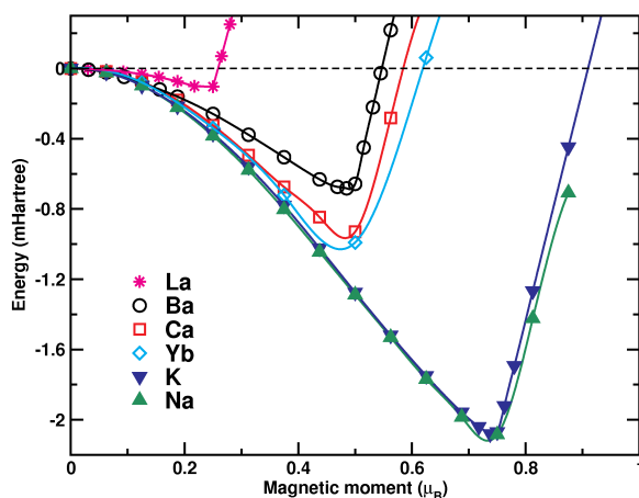
Fig. 7: Relative energy vs. magnetic moment per Fe-atom resulting from fixed spin moment (FSM) calculations for various filled skutterudites M\text{Fe}_4\text{Sb}_{12} ( M = \text{Na}, \text{K}, \text{Ca}, \text{Ba}, \text{La}, \text{Yb} ; 1 Hartree \approx 27.2 eV).
