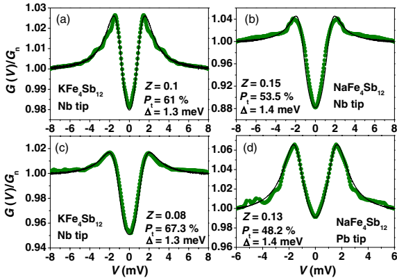
Fig. 11: Selected conductance spectra G(V) for the skutterudites KFe_4Sb_{12} (a,c) and NaFe_4Sb_{12} (b,d) taken at 2.8 K. The spectra were measured (dots) using (a-c) Nb or (d) Pb tips and were normalized to the normal state conductance G_n at high voltage. The lines present the results of the best fits with the fit parameters given in each panel (see text).
