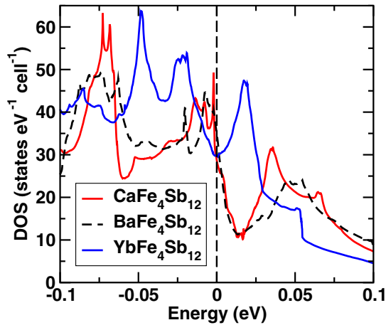
Fig. 10: Total density of states of M\text{Fe}_4\text{Sb}_{12} near the Fermi level E_F . For M = \text{Yb} , the scalar relativistic result is shown without spin-orbit coupling. For M = \text{Ca}, \text{Ba} the spin orbit coupling was included leading to an upward shift as well as to a broadening of the peak \approx 50 meV above E_F .
