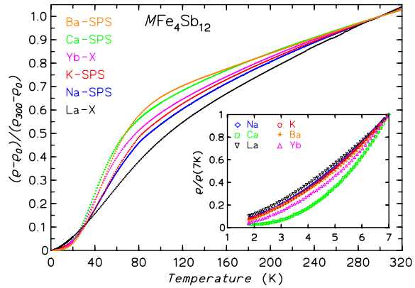
Fig. 5: Normalized electrical resistivity of filled skutterudites M\text{Fe}_4\text{Sb}_{12} ( M = \text{Na}, \text{K}, \text{Ca}, \text{Ba}, \text{La}_{1-x}, \text{Yb}_{1-x} ). X assigns single crystal samples (La, Yb), all other samples are spark plasma sintered (SPS) material. The inset shows data below 7 K.
