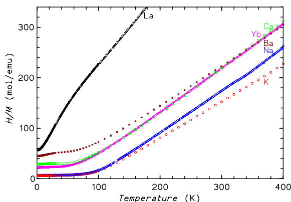
Fig. 6: Inverse magnetic susceptibility H/M(T) of filled skutterudites M\text{Fe}_4\text{Sb}_{12} with various cations M = \text{Na}, \text{K}, \text{Ca}, \text{Ba}, \text{La}, \text{Yb} .
