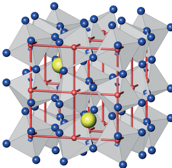
Fig. 1: Cubic unit cell of iron-antimony skutterudites M\text{Fe}_4\text{Sb}_{12} containing two formula units (yellow spheres M = \text{alkali, alkaline-earth, rare-earth metal} ; red spheres \text{Fe} ; blue spheres \text{Sb} ).
