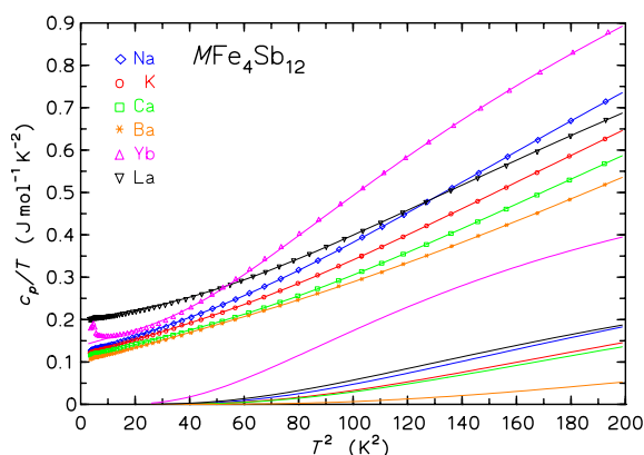
Fig. 3: Specific heat capacity of filled skutterudites M\text{Fe}_4\text{Sb}_{12} ( M = \text{Na}, \text{K}, \text{Ca}, \text{Ba}, \text{La}_{0.79}, \text{Yb}_{0.95} ) below 14 K in a c_p/T vs. T^2 representation. The lines show the fits of the model described in the text.
