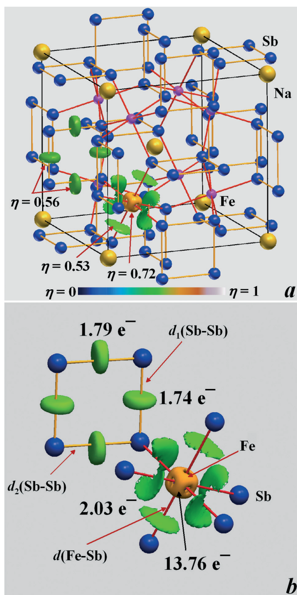
Fig. 2: Electron localization function \eta for \text{NaFe}_4\text{Sb}_{12} . (a) Crystal structure of \text{NaFe}_4\text{Sb}_{12} with shortest interatomic distances Fe-Sb and Sb-Sb. Isosurfaces of ELF illustrate the covalent interaction between Fe and Sb ( \eta = 0.53 ) and between Sb atoms ( \eta = 0.56 ). The isosurface for \eta = 0.72 shows the structuring of the third shell for the Fe atoms; see text. (b) Electron counts for relevant bonds in the \text{NaFe}_4\text{Sb}_{12} structure.
