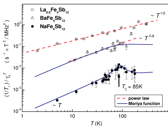
Figure 8: 1/T_1 normalized to the nuclear gyromagnetic ratio \gamma_N^2 as a function of temperature as obtained from ^{139}\text{La} -NMR ( ^{139}\gamma_N = 6.014 MHz/T), ^{137}\text{Ba} -NQR ( ^{137}\gamma_N = 4.731 MHz/T, from the \nu_1 -line) and ^{23}\text{Na} -NMR ( ^{23}\gamma_N = 11.262 MHz/T). The solid line is a calculation of 1/T_1 vs. T based on Moriya's theory [21], making use of the field- and temperature-dependent magnetization M(H,T) for weak itinerant ferromagnets. The dashed line is a fit to a T^{1/2} power law.
