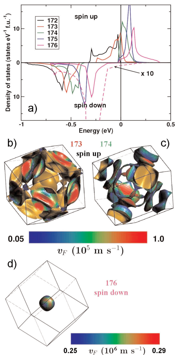
Fig. 13: Calculated density of states (DOS) and Fermi surfaces for \text{KFe}_4\text{Sb}_{12} . (a) DOS resolved for the individual bands relevant at E_F . Spin-down band 176 has a non-vanishing DOS at E_F (cf. dashed line that represents a factor of 10 magnification). (b,c) Fermi surfaces for the most contributing spin-up bands 173 (b) and 174 (c). The color coding indicates the Fermi velocities v_F . (d) Fermi surface and velocity for the relevant spin-down band 176.
